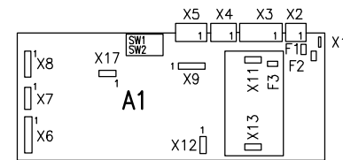
CONTROL CIRCUIT (COMPONENTS SIDE) CIRCUITO MANDO (LADO COMPONENTES) CIRCUIT COMMANDE (COTE COMPOSANTS)
